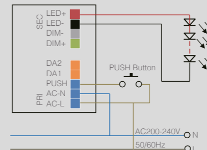
Wiring diagram for PUSH DIM
