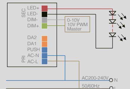
Wiring diagram for 0-10V, or 10V PWM
